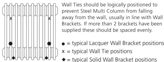
Fig 1 - Bracket Positions
